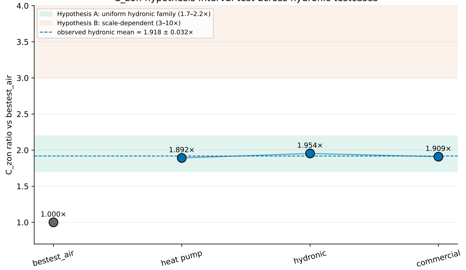
C_zon hypothesis interval test across hydronic testcases
