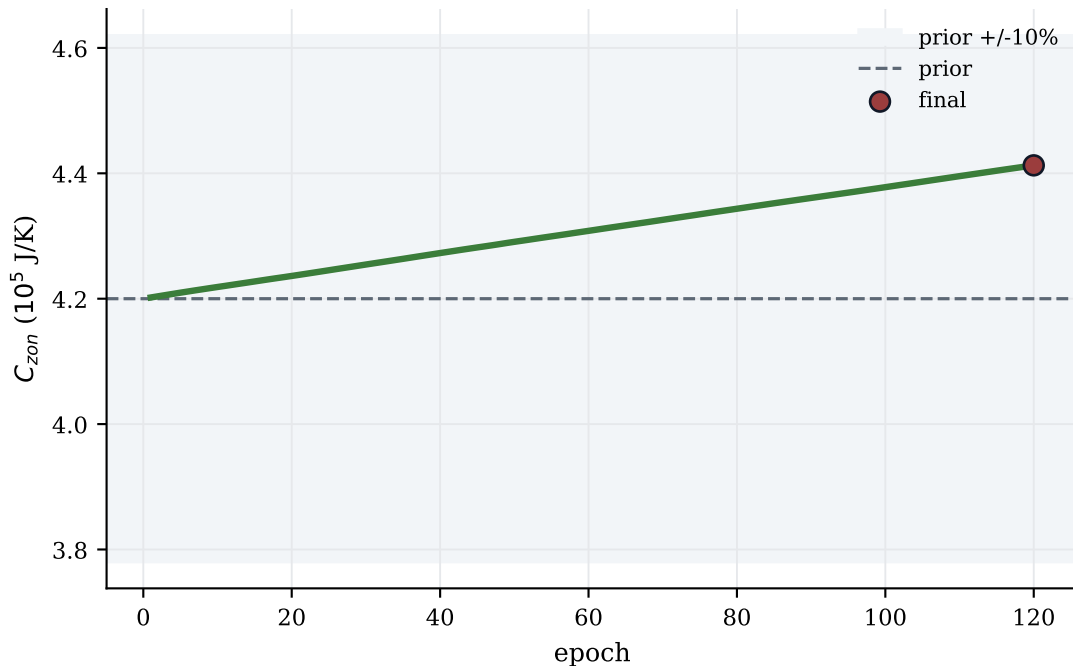
(a) Stage B physical-parameter identification
