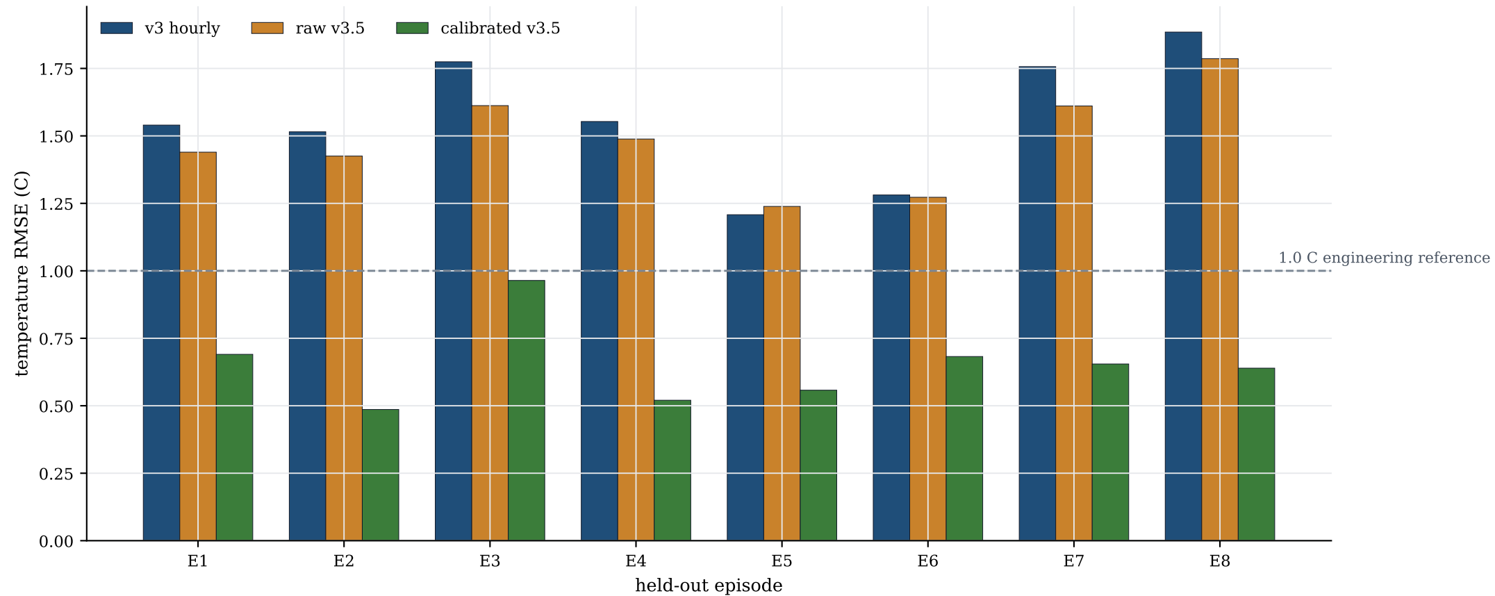
Replicative validity across held-out BOPTEST episodes
