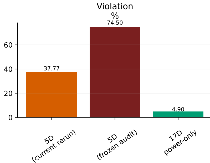
MORL observation-interface ablation: 5D failure (current rerun and frozen audit) → 17D success
