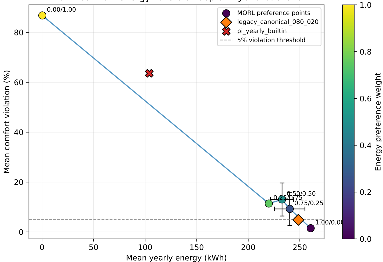
MORL comfort-energy Pareto sweep on hybrid backend
