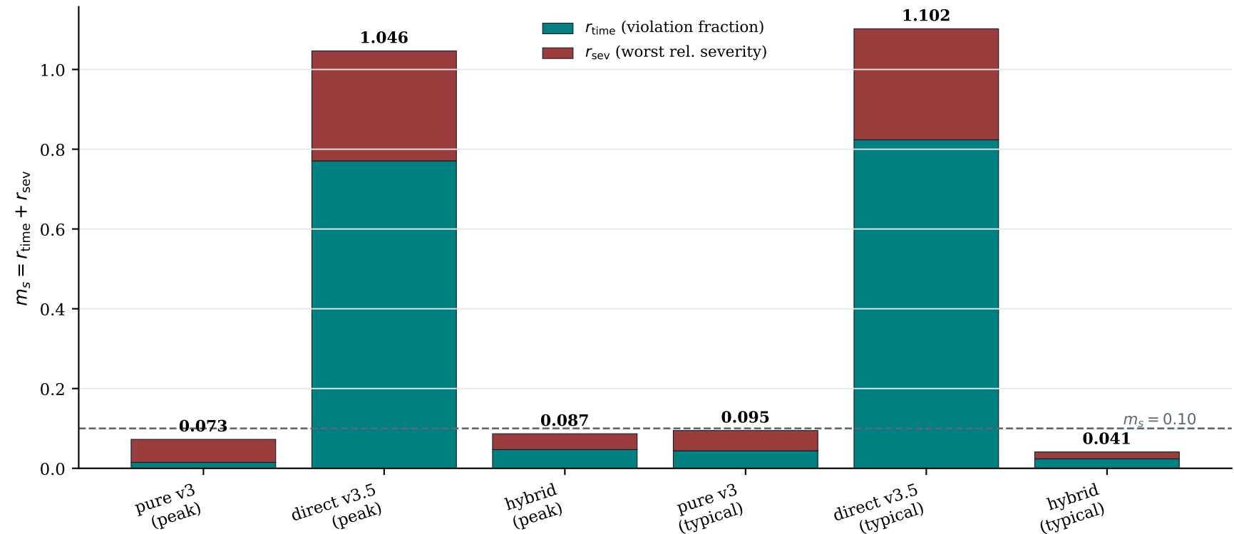
Maintenance-score decomposition on the live BOPTEST windows
