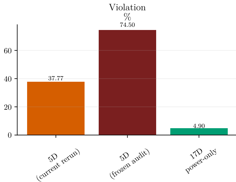
MORL observation-interface ablation: 5D failure (current rerun and frozen audit) \rightarrow 17D success
