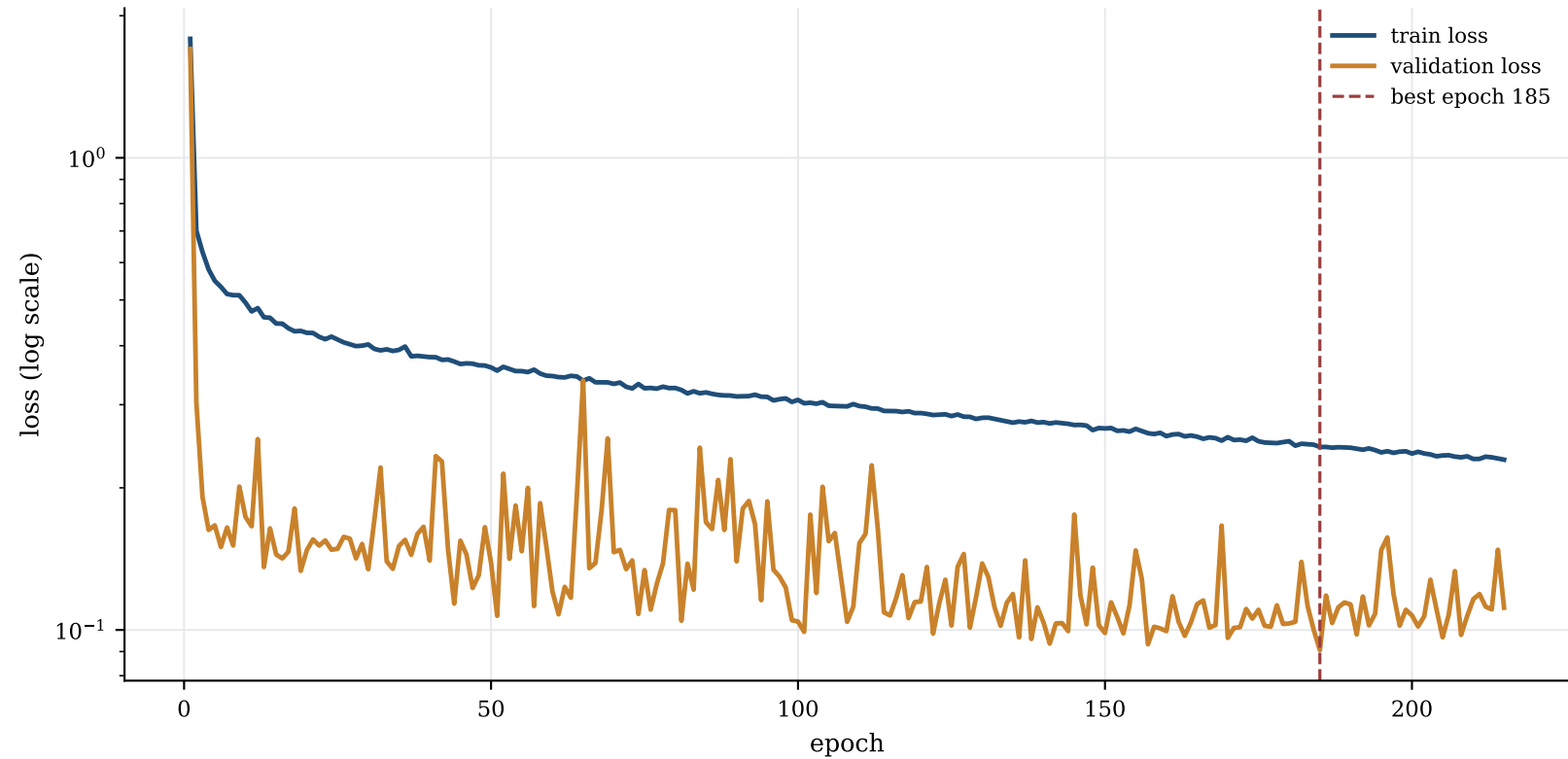
v3 supervised learning curves
