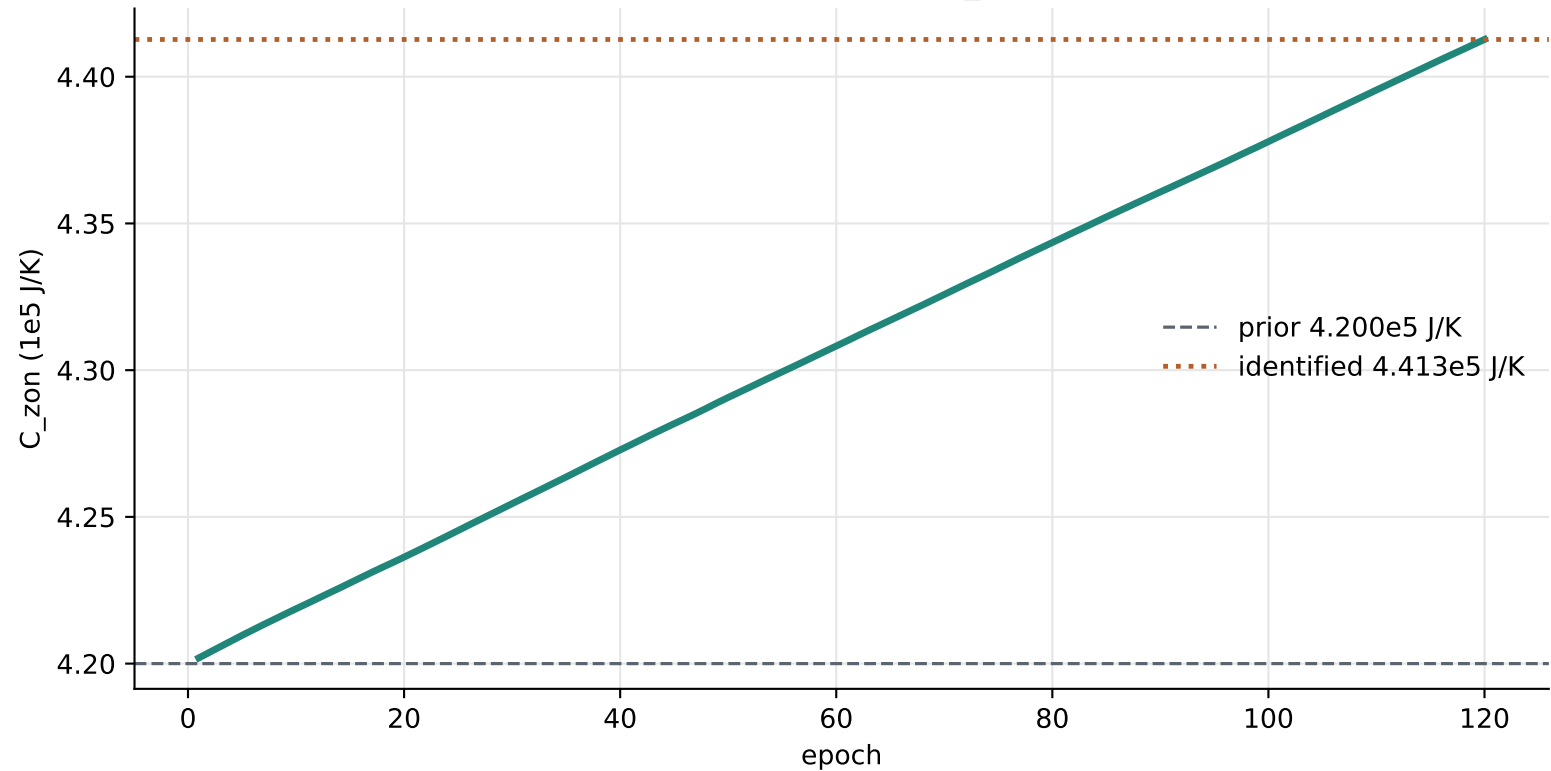
Bayesian inverse identification trajectory of C_{zon} during Stage B
