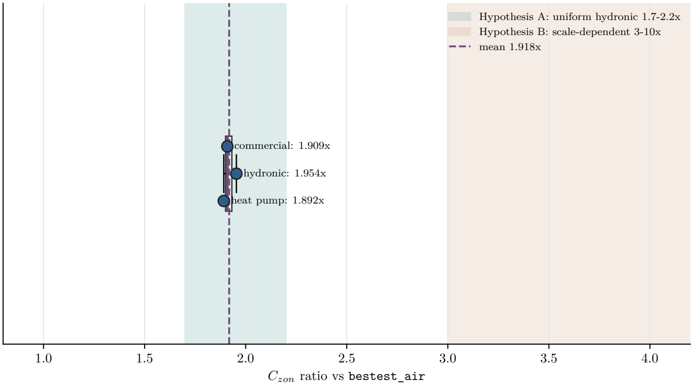
C_{zon} hydronic-family consistency against version-locked hypothesis intervals
