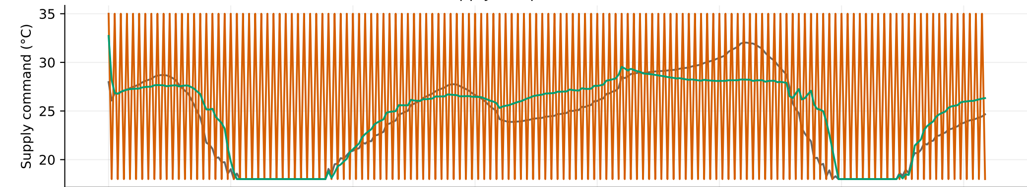
(b) Supply-temperature command
