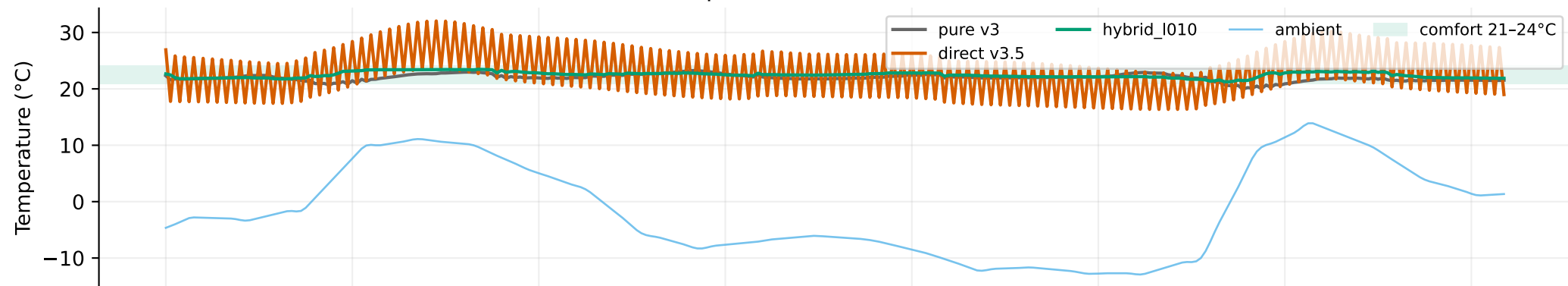
(a) Zone temperature and ambient disturbance
