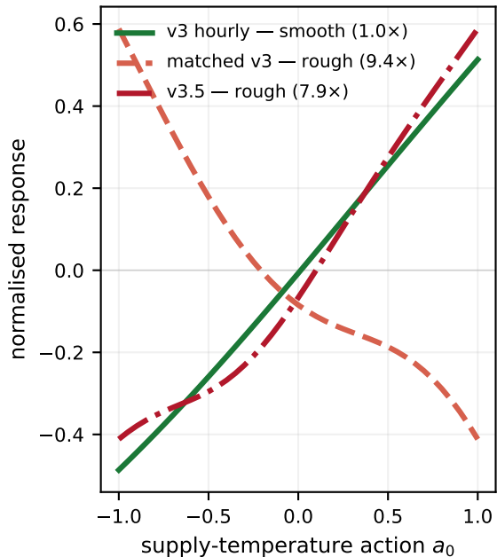
(A) Action \rightarrow next-temperature shape
