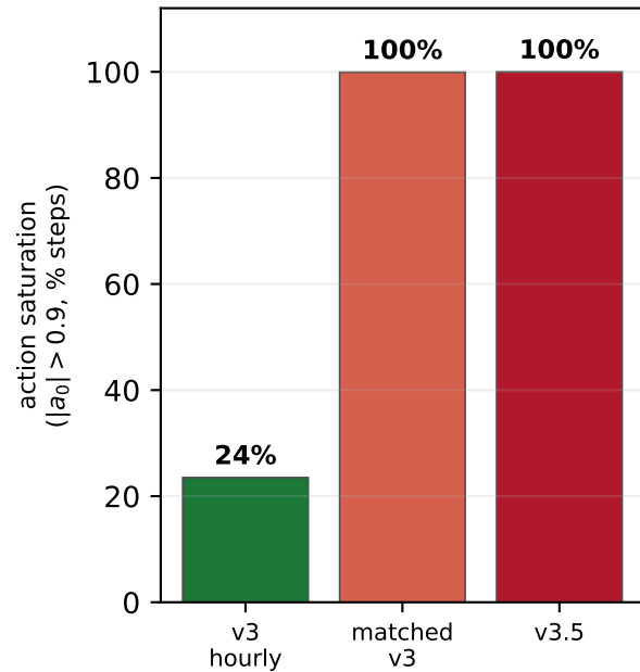
(C) Live policy bang-bang
