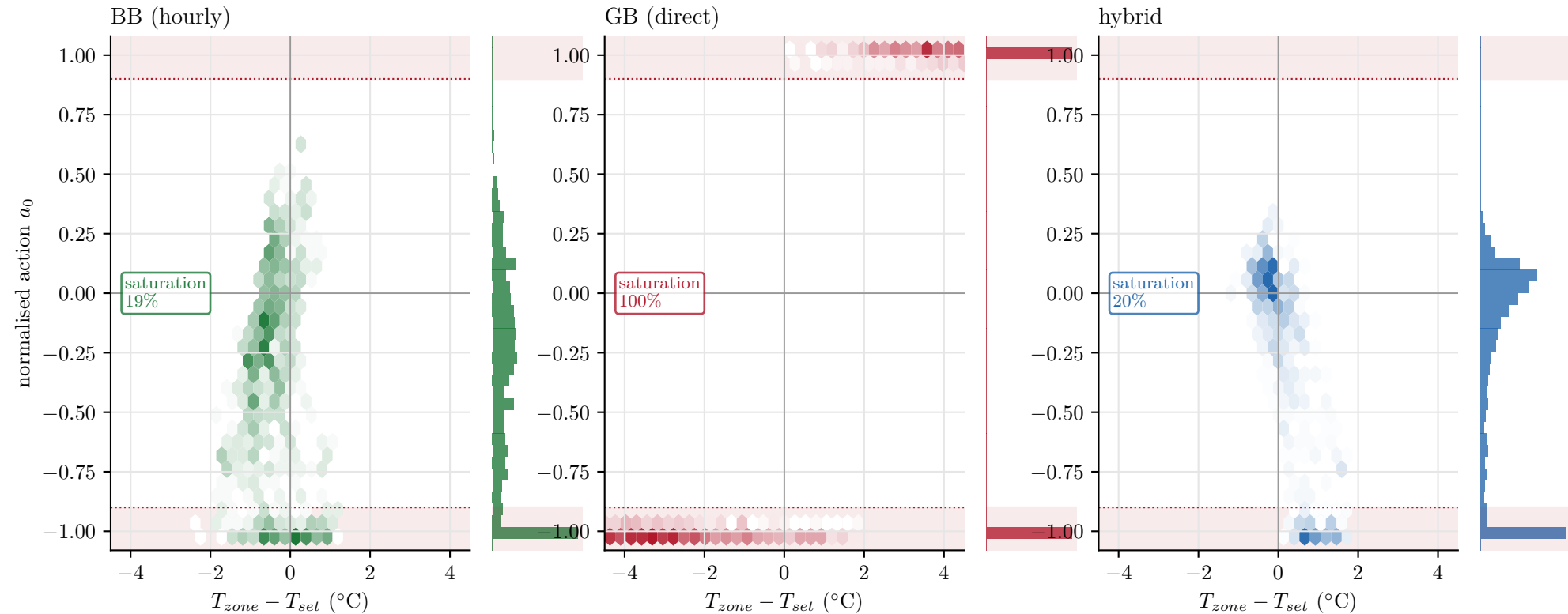
Action-density phase portrait: policy action vs thermal error (identical axes; red bands = saturation |a_0| \geq 0.9 ; right strip = marginal a_0 )
