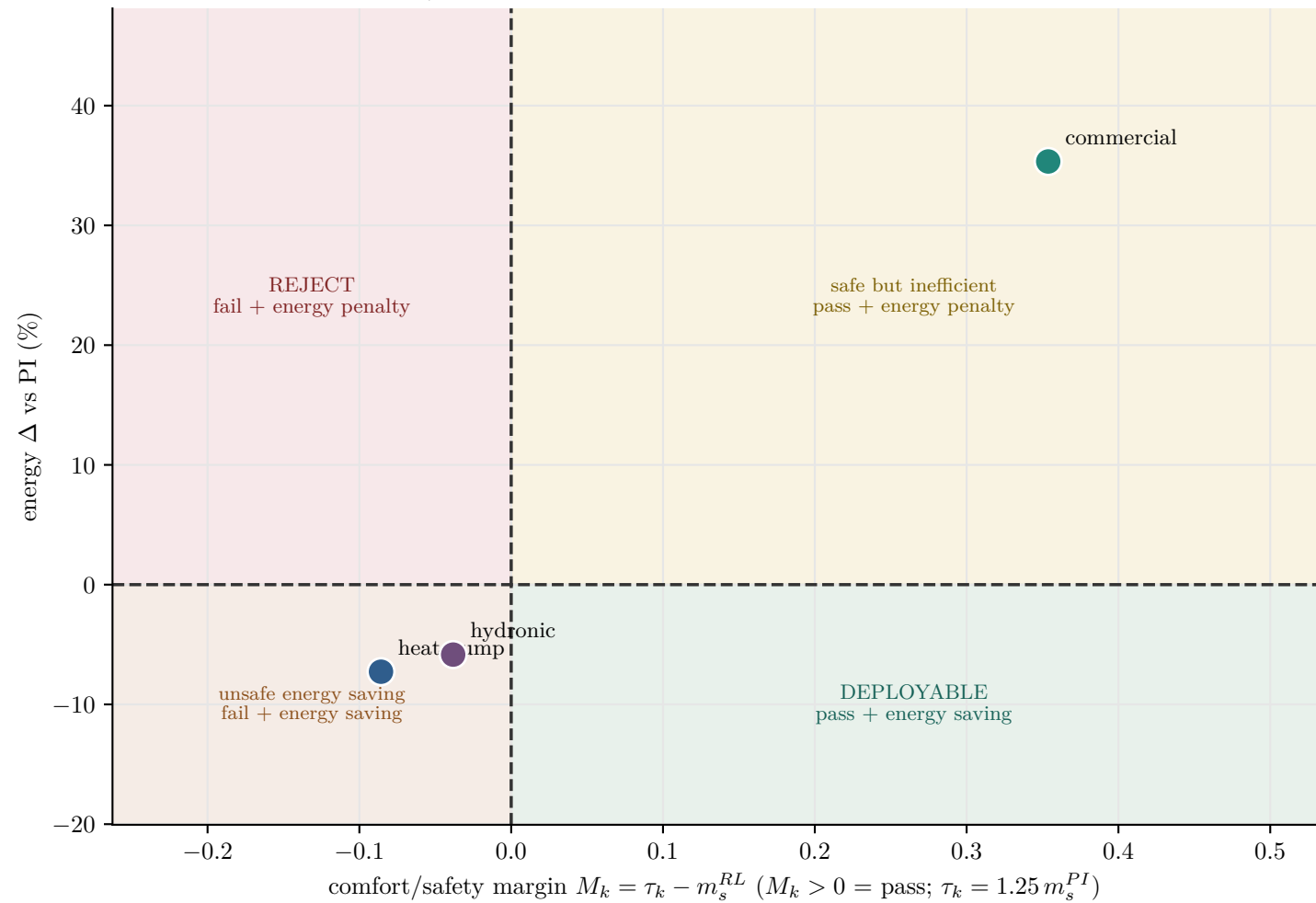
Deployment plane: comfort/safety margin vs energy
