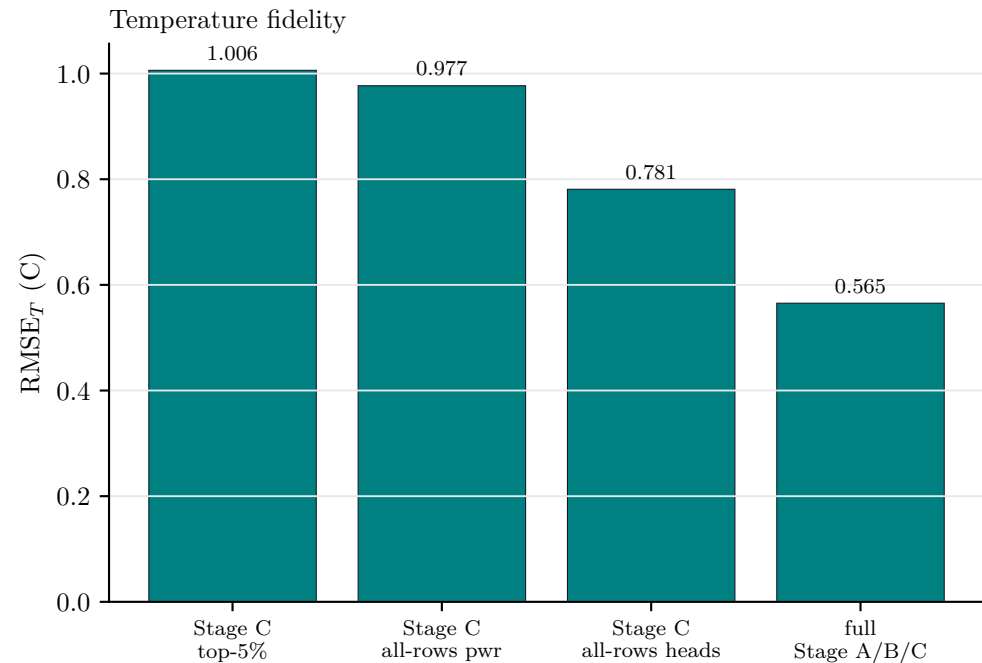
Primary testcase: surrogate fidelity improves with recalibration depth (controller frozen)
