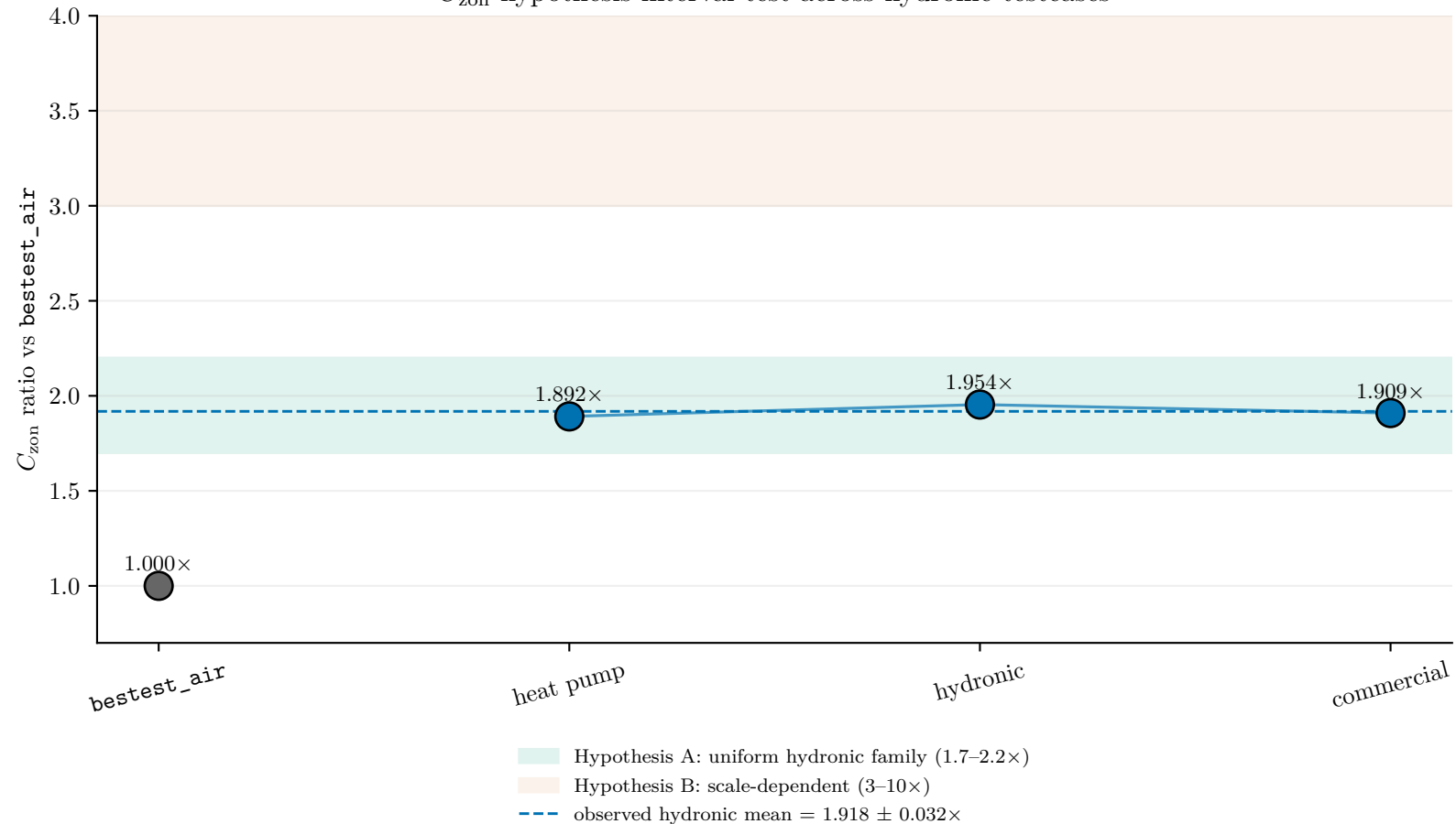
C_{\text{zon}} hypothesis interval test across hydronic testcases
