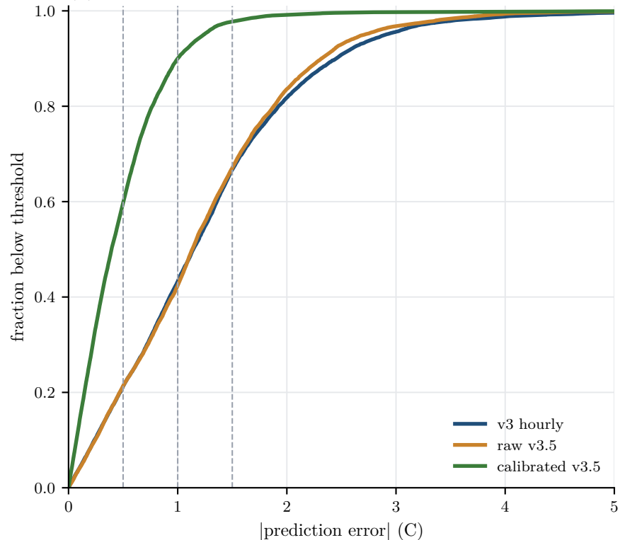
(b) Engineering tolerance CDF
