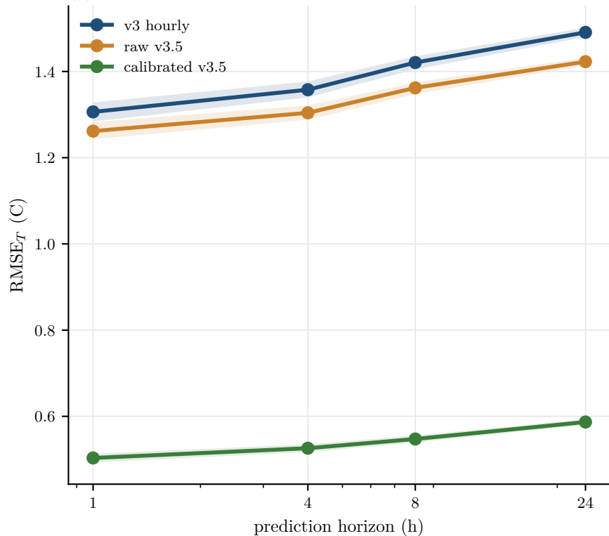
(a) Multi-horizon rollout RMSE
