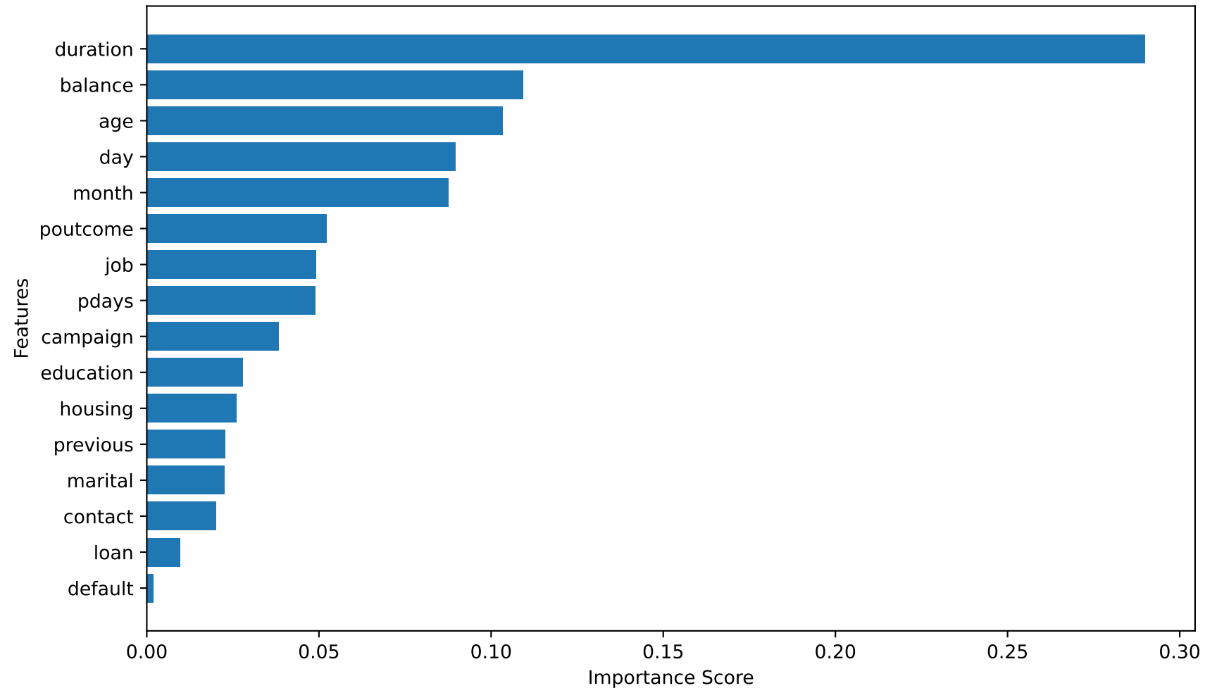
Feature Importance using Random Forest
