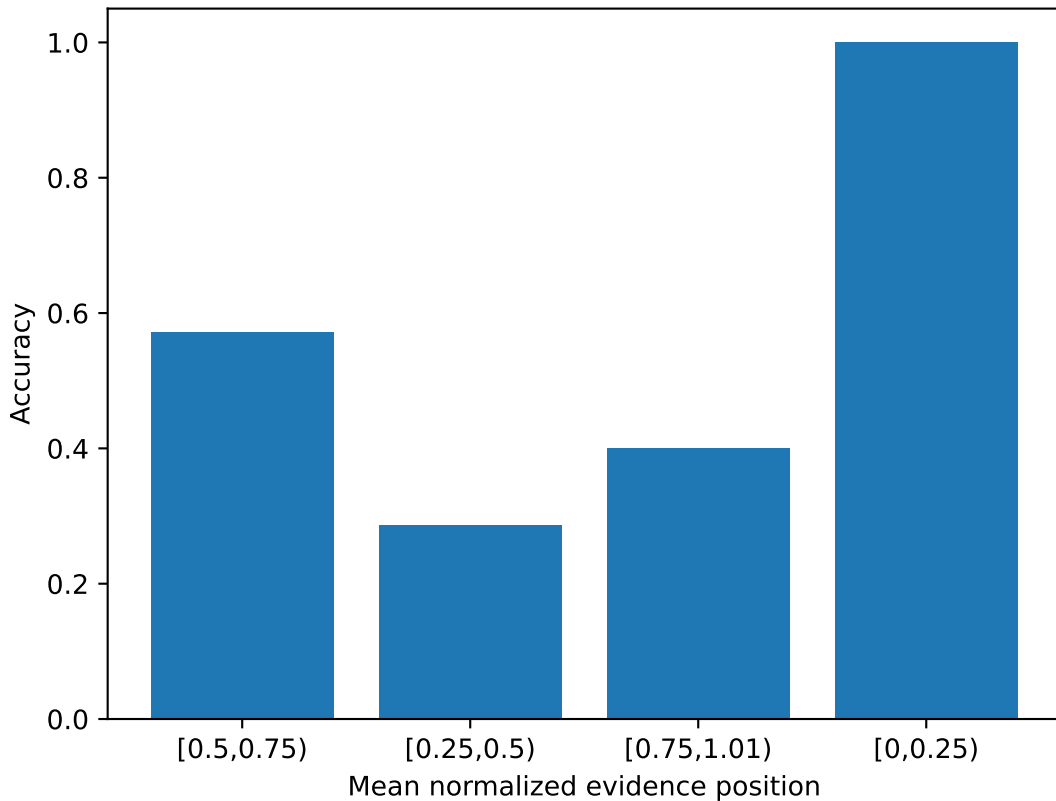
Accuracy vs. mean normalized evidence position
