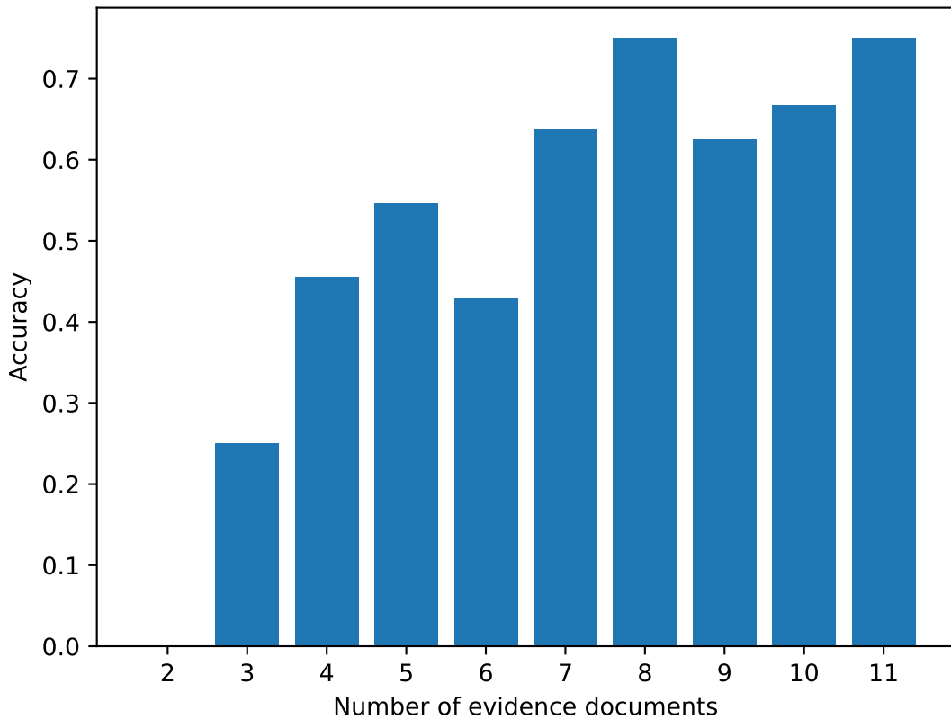
Accuracy vs. number of evidence documents
