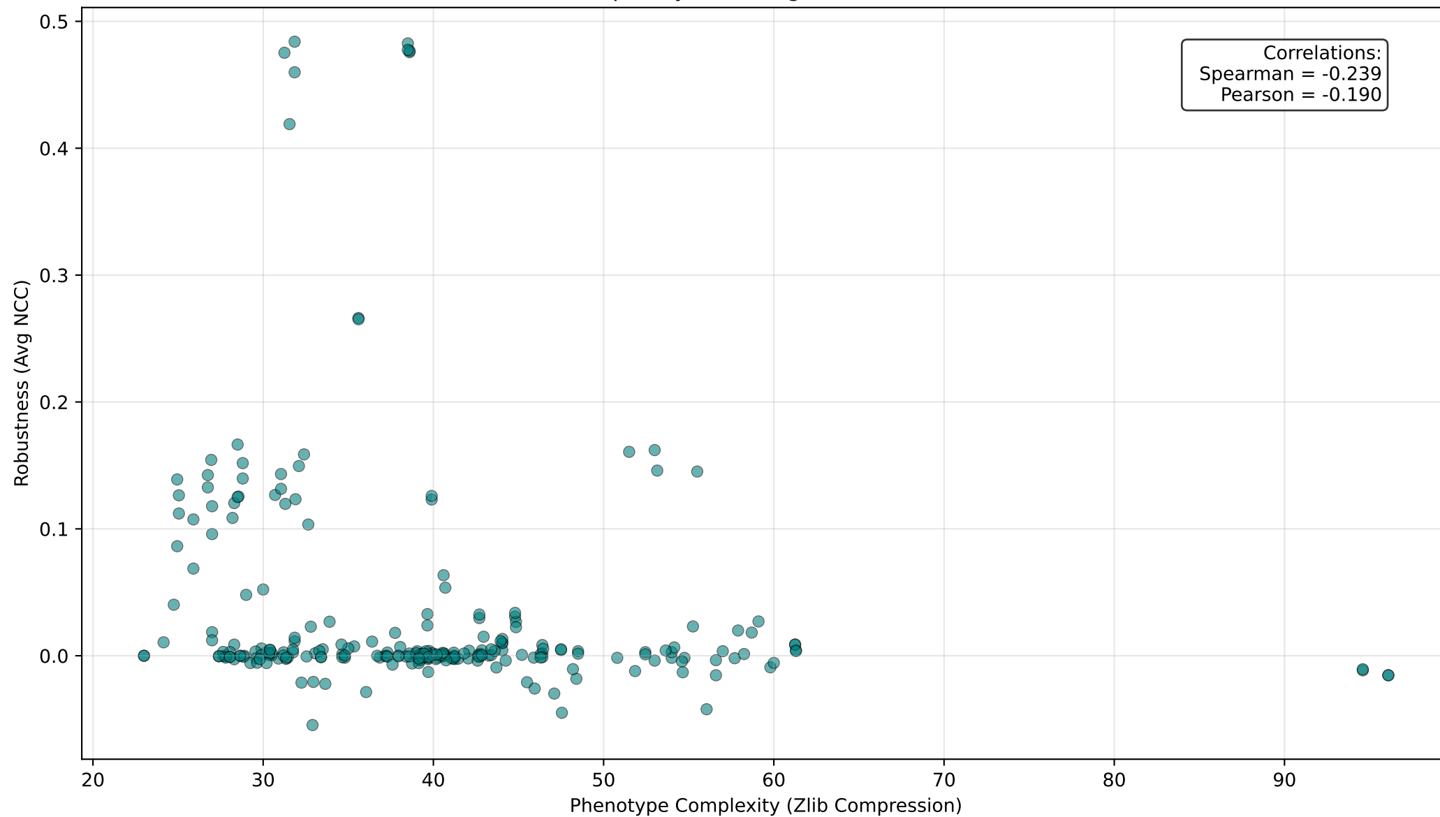
1D CA Robustness VS Complexity, Mutating Seeds, Shuffled Control. L=8, T=256
