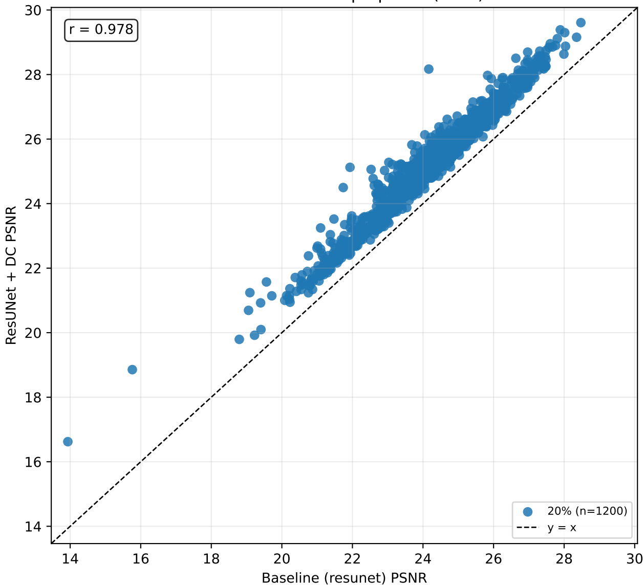
PSNR baseline vs proposed (axial)
