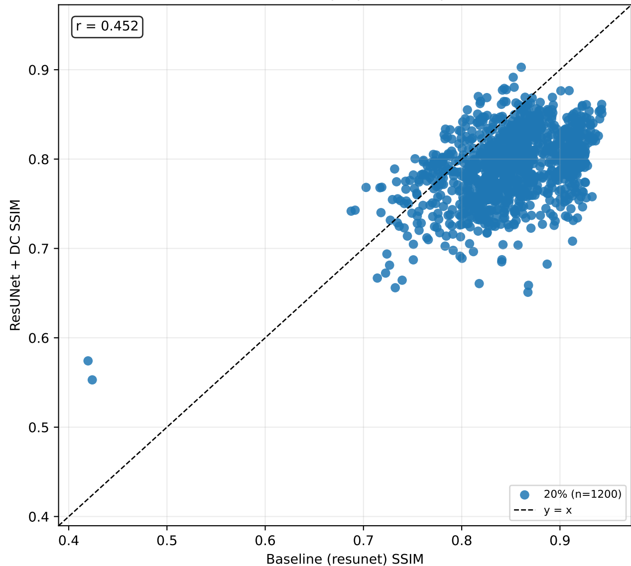
SSIM baseline vs proposed (all planes)
