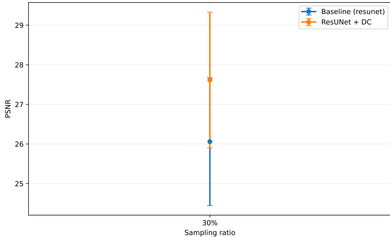
PSNR vs sampling ratio (axial)
