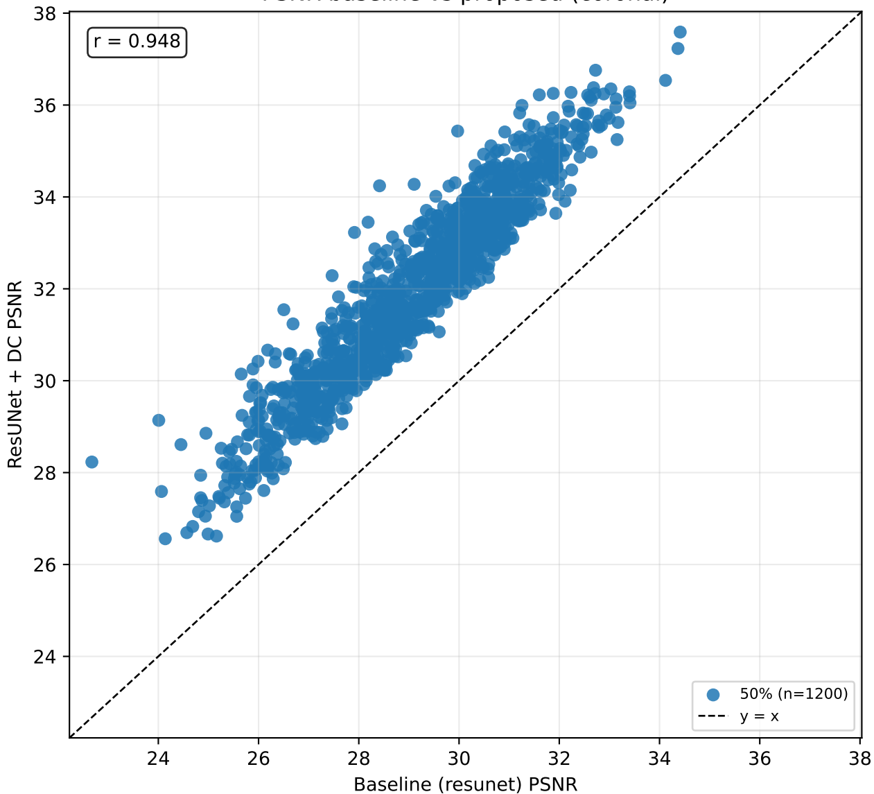
PSNR baseline vs proposed (coronal)
