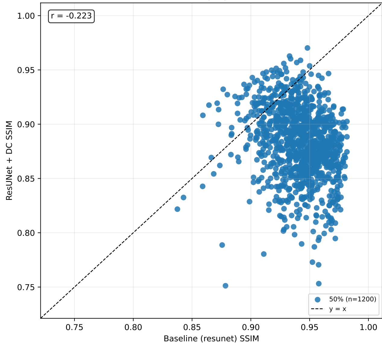
SSIM baseline vs proposed (coronal)
