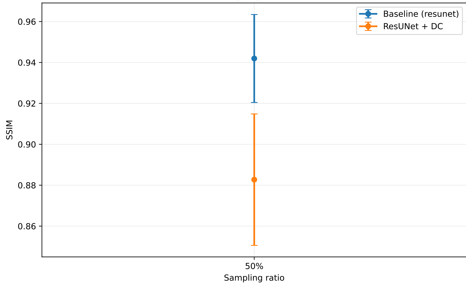
SSIM vs sampling ratio (coronal)
