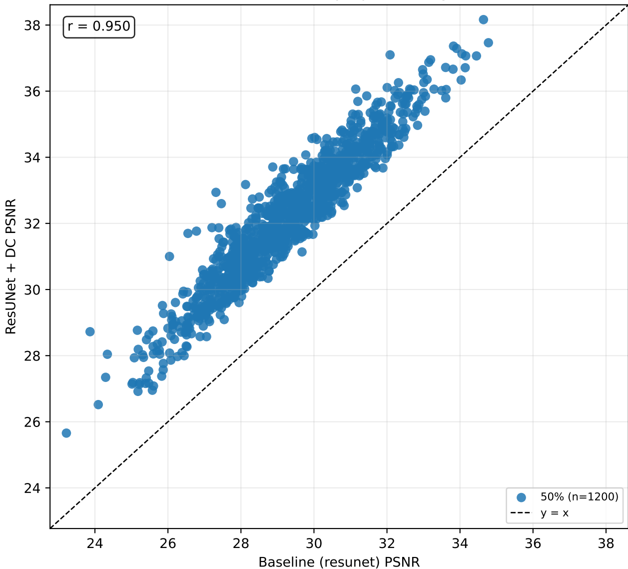
PSNR baseline vs proposed (sagittal)
