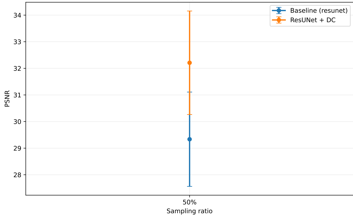
PSNR vs sampling ratio (sagittal)
