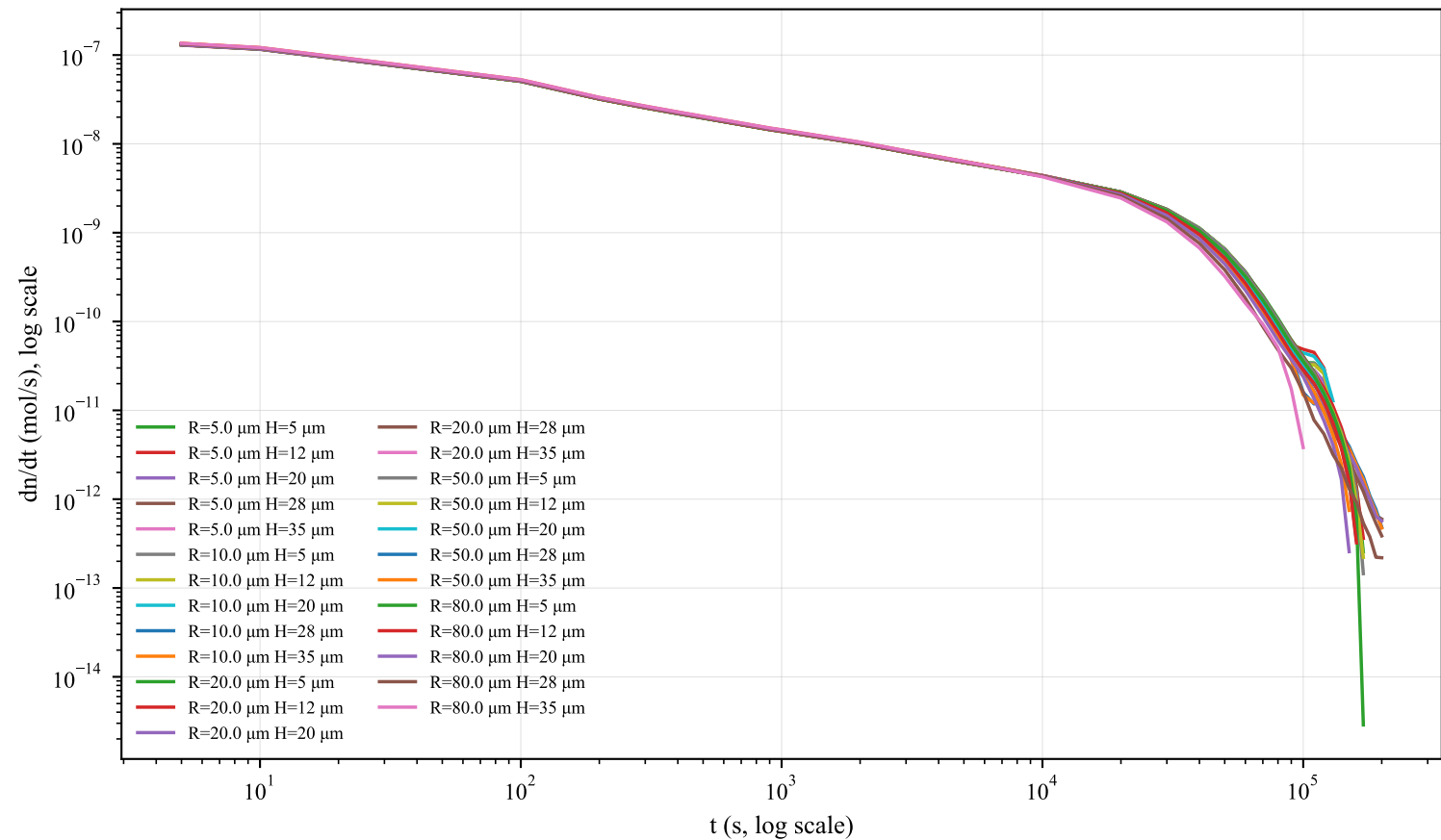
Adsorption rate over time -- cone_recessed ( t \geq 5s )
