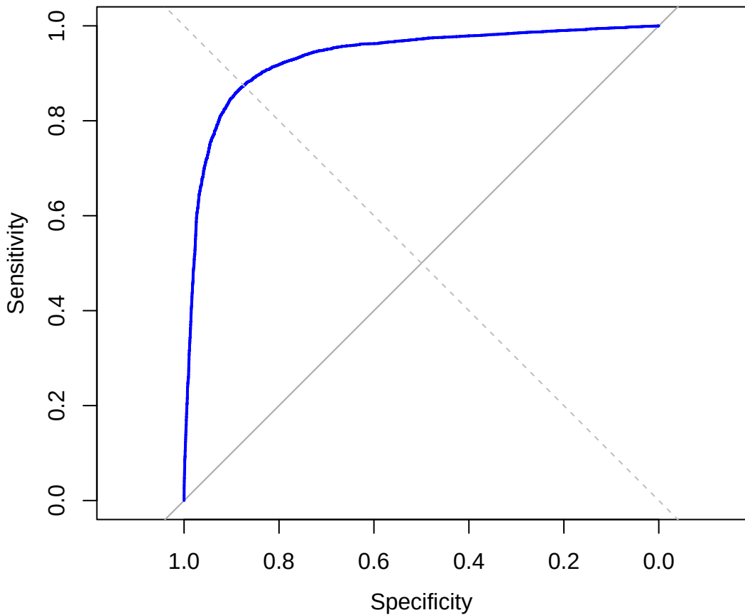
Logistic Regression ROC (TEST AUC=0.9335)
