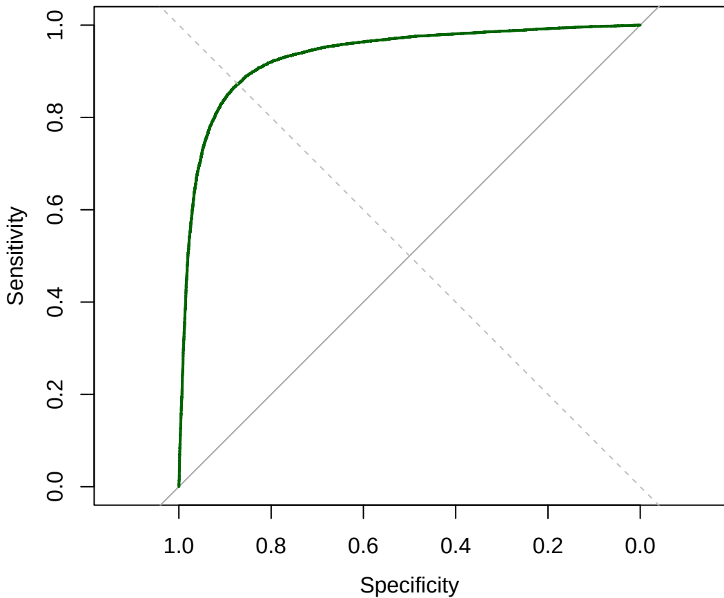
Logistic Regression ROC (TRAIN AUC=0.9337)
