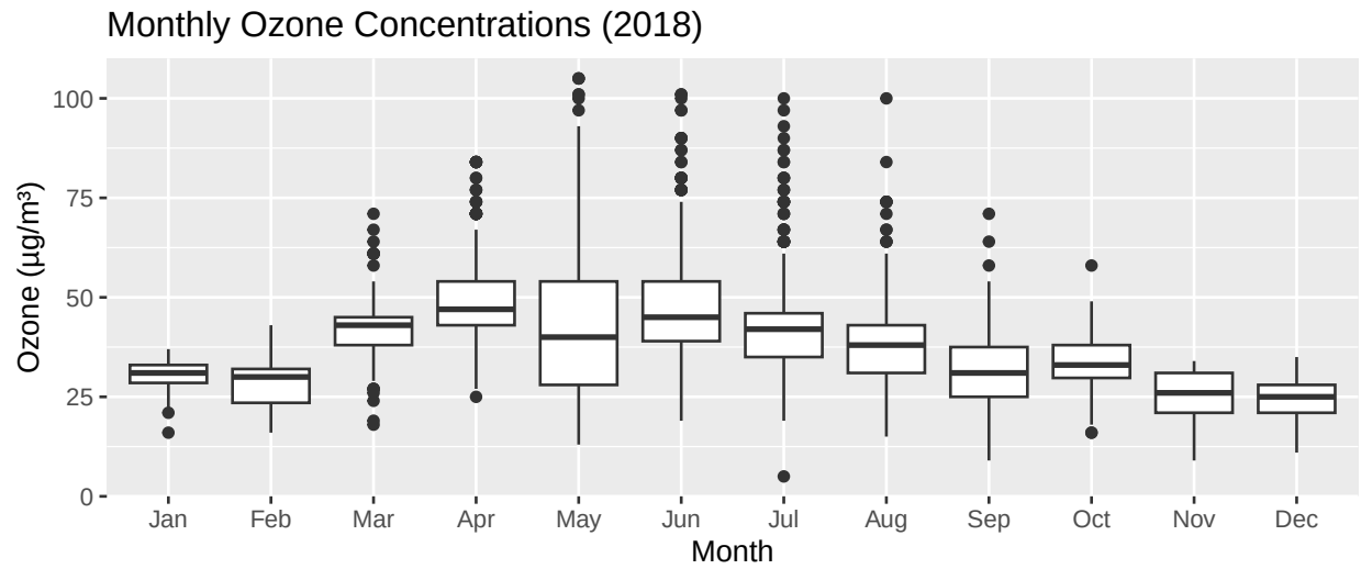
Figure 1: Monthly Ozone Concentrations (2018) Boxplot
