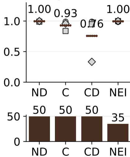
synthetic
