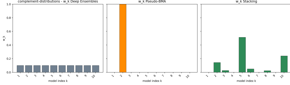
Figure 5: Complement-distributions task: Pseudo-BMA collapses onto model 2 ( w_2 \approx 1 ), while stacking distributes weight across models 2, 5, 6, and 10.
