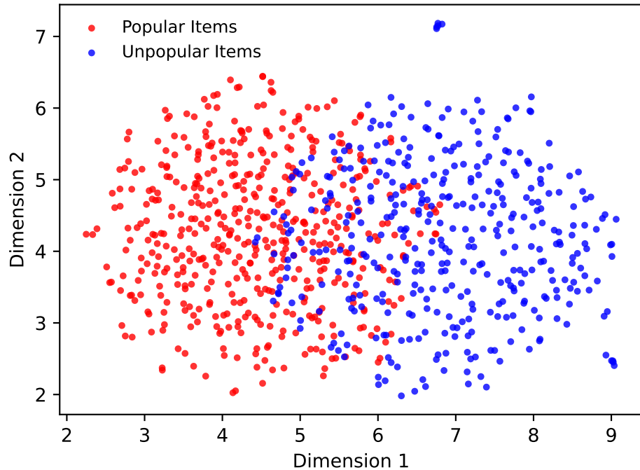
(b) Item Visualization Updated Embeddings
