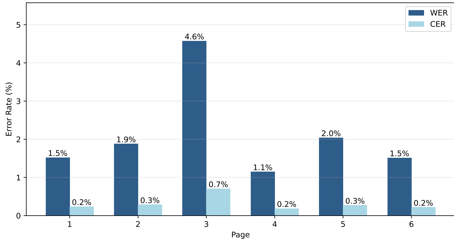
Experiment 2 (English) - Qwen3.5-35B-A3B
