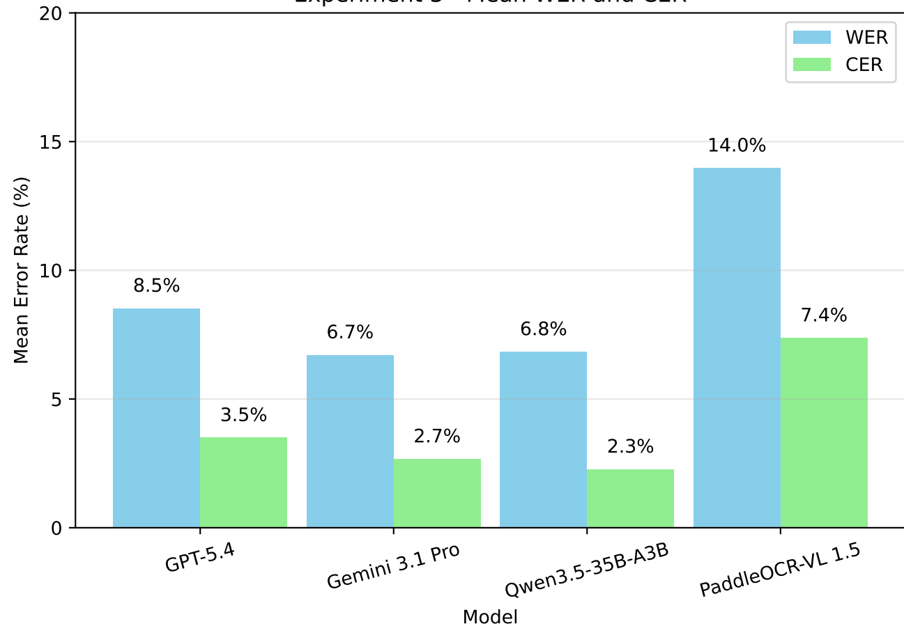
Experiment 3 - Mean WER and CER
