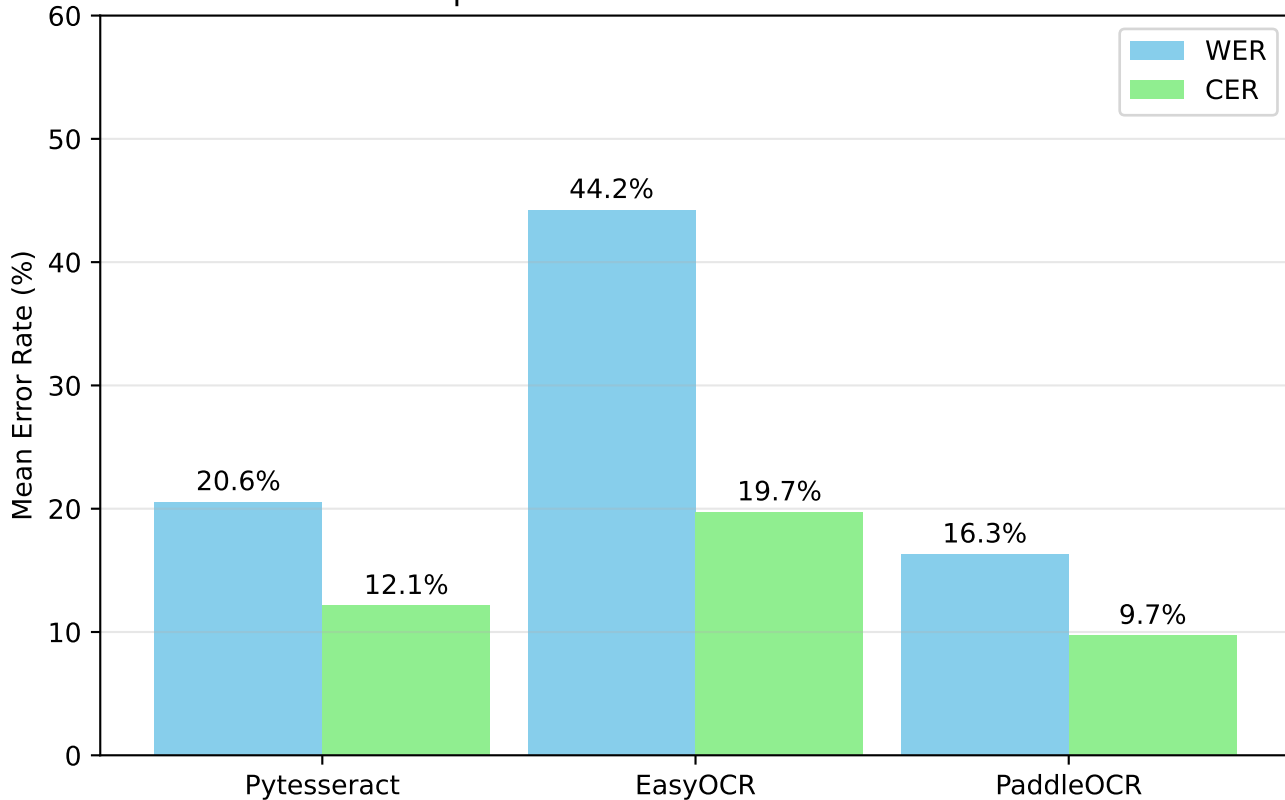
Experiment 3 - Mean WER and CER
