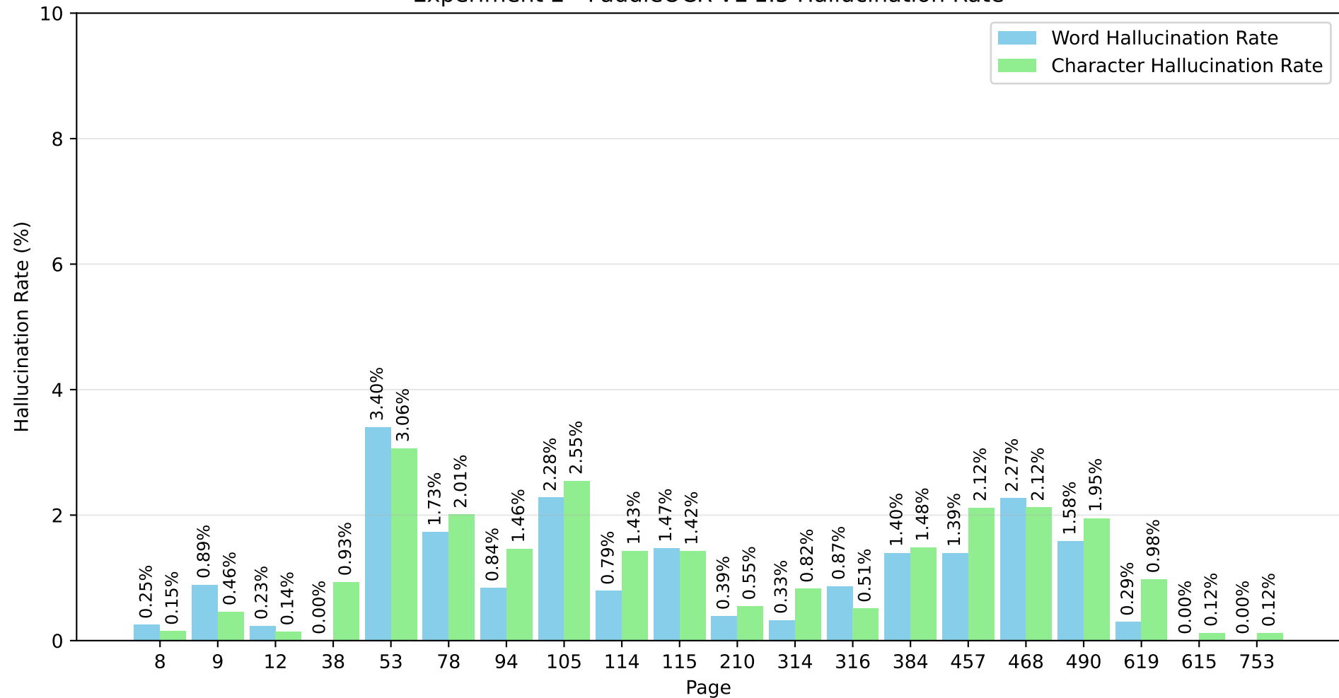
Experiment 2 - PaddleOCR-VL 1.5 Hallucination Rate
