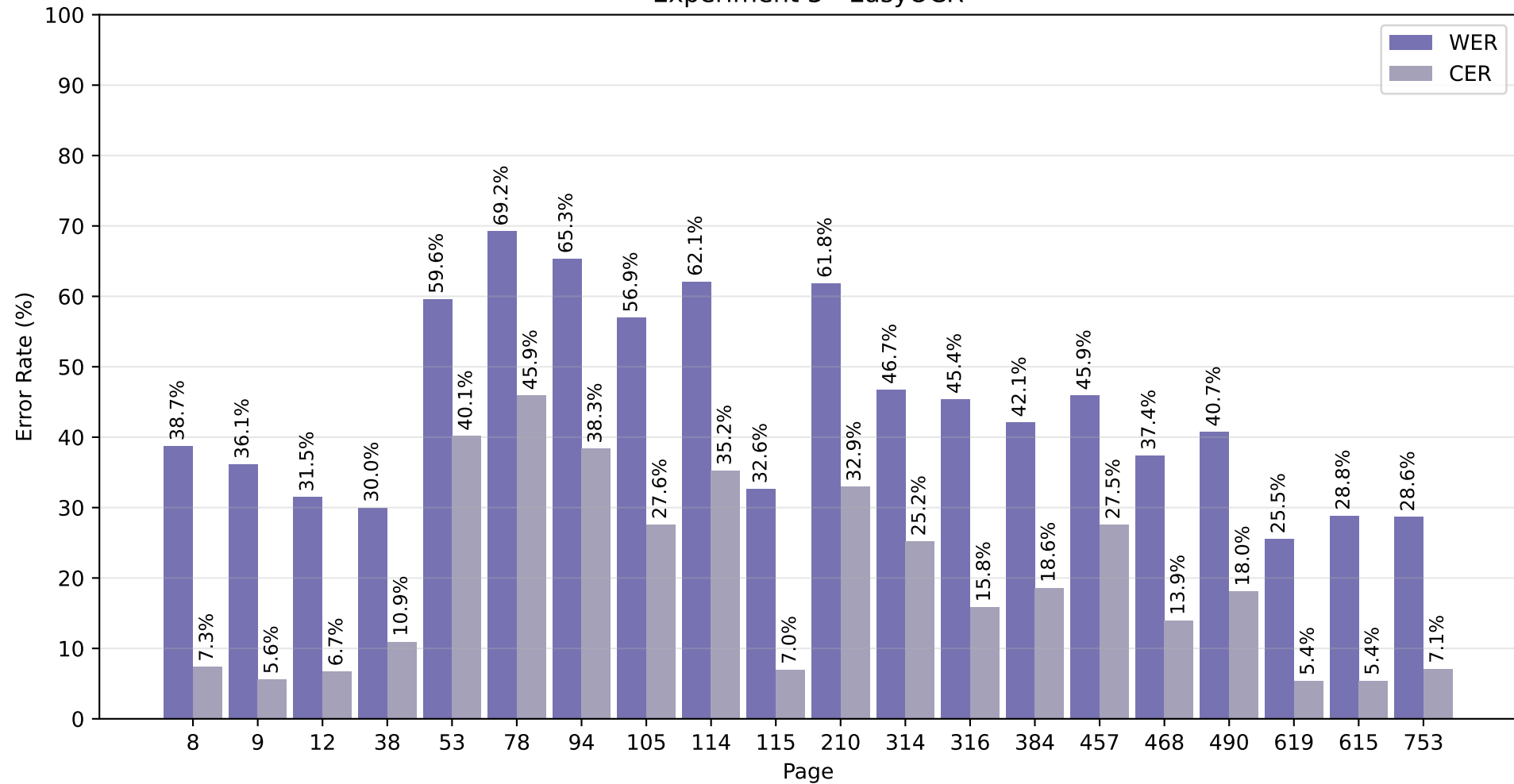
Experiment 3 - EasyOCR
