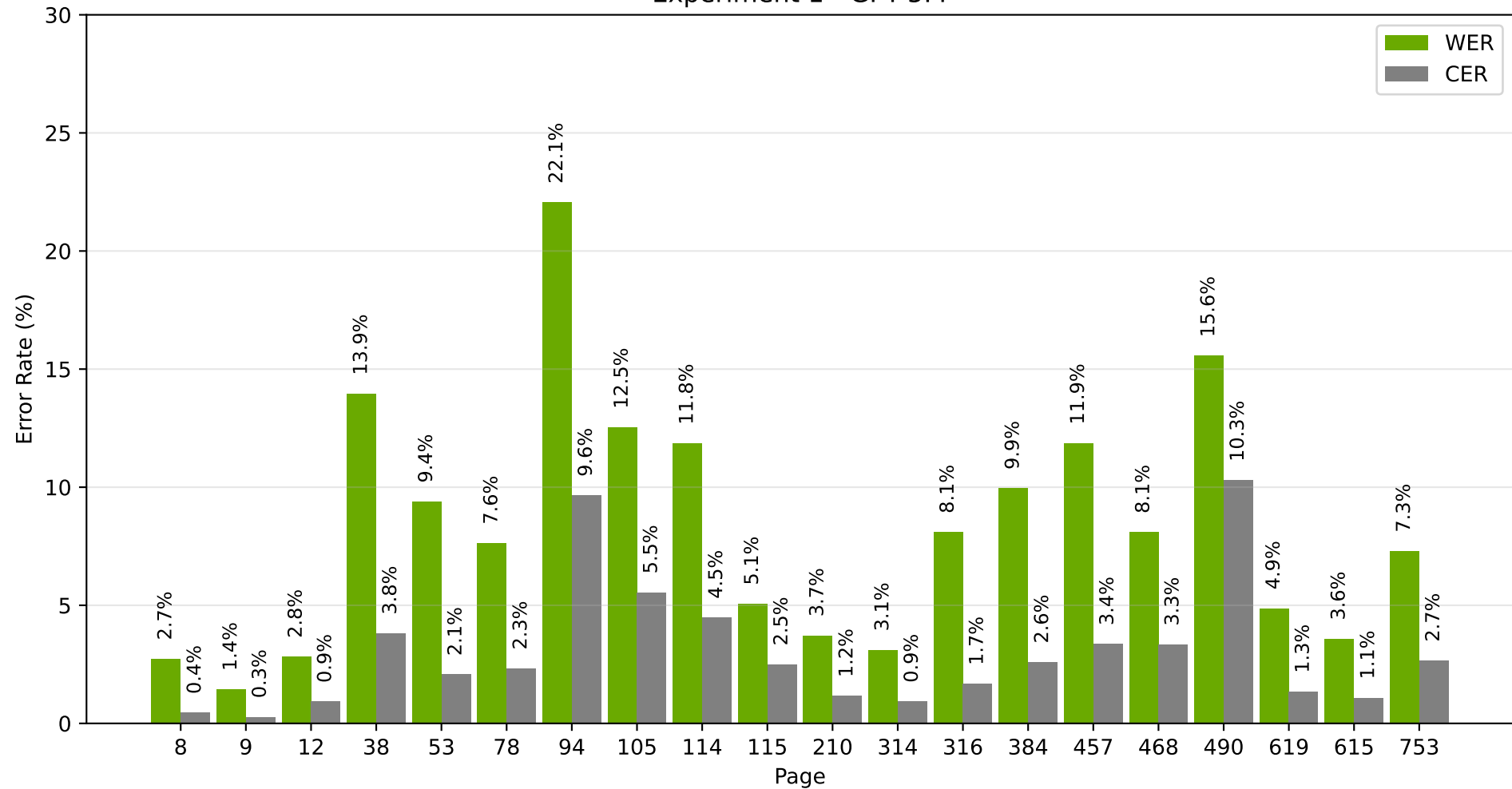
Experiment 1 - GPT-5.4
