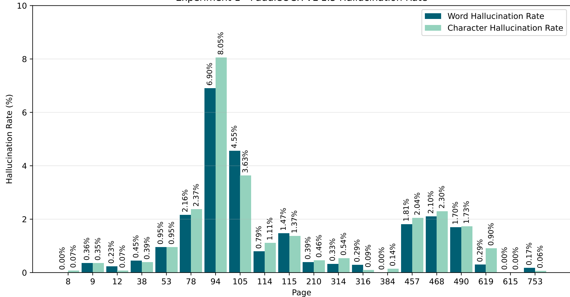
Experiment 1 - PaddleOCR-VL 1.5 Hallucination Rate
