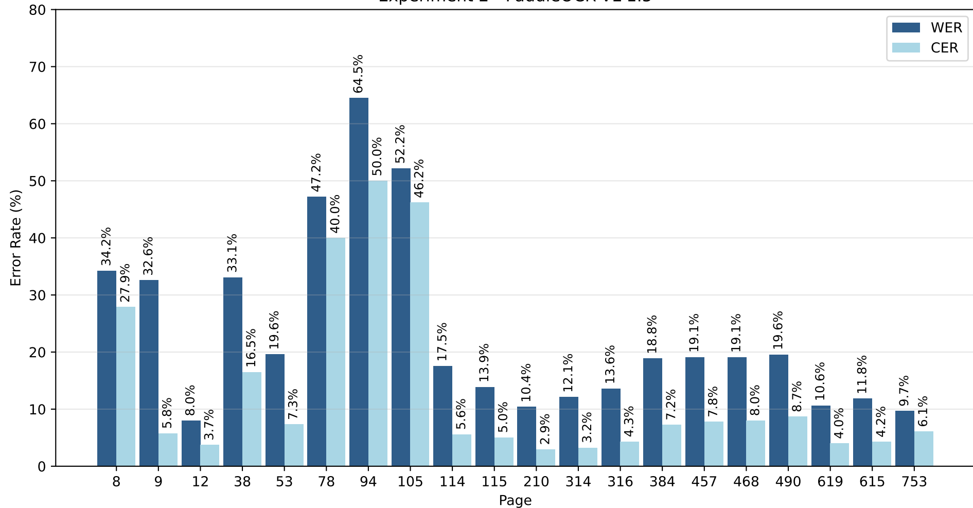
Experiment 2 - PaddleOCR-VL 1.5
