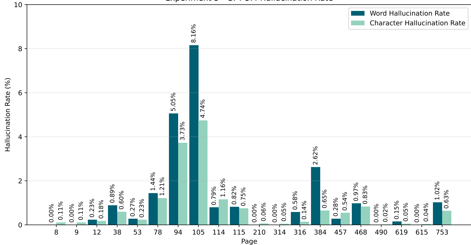
Experiment 3 - GPT-5.4 Hallucination Rate
