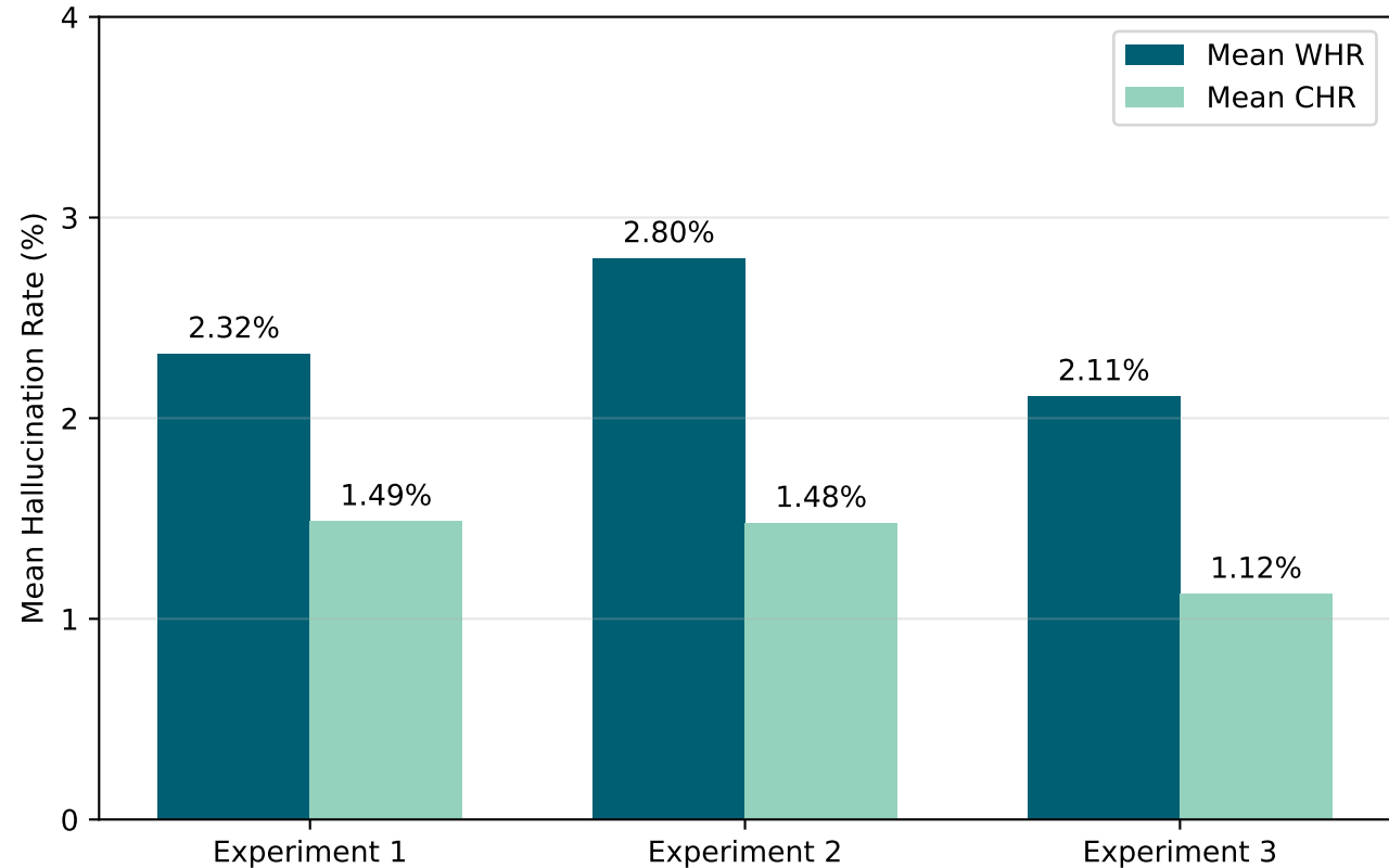
Gemini 3.1 Pro Mean Hallucination Rate
