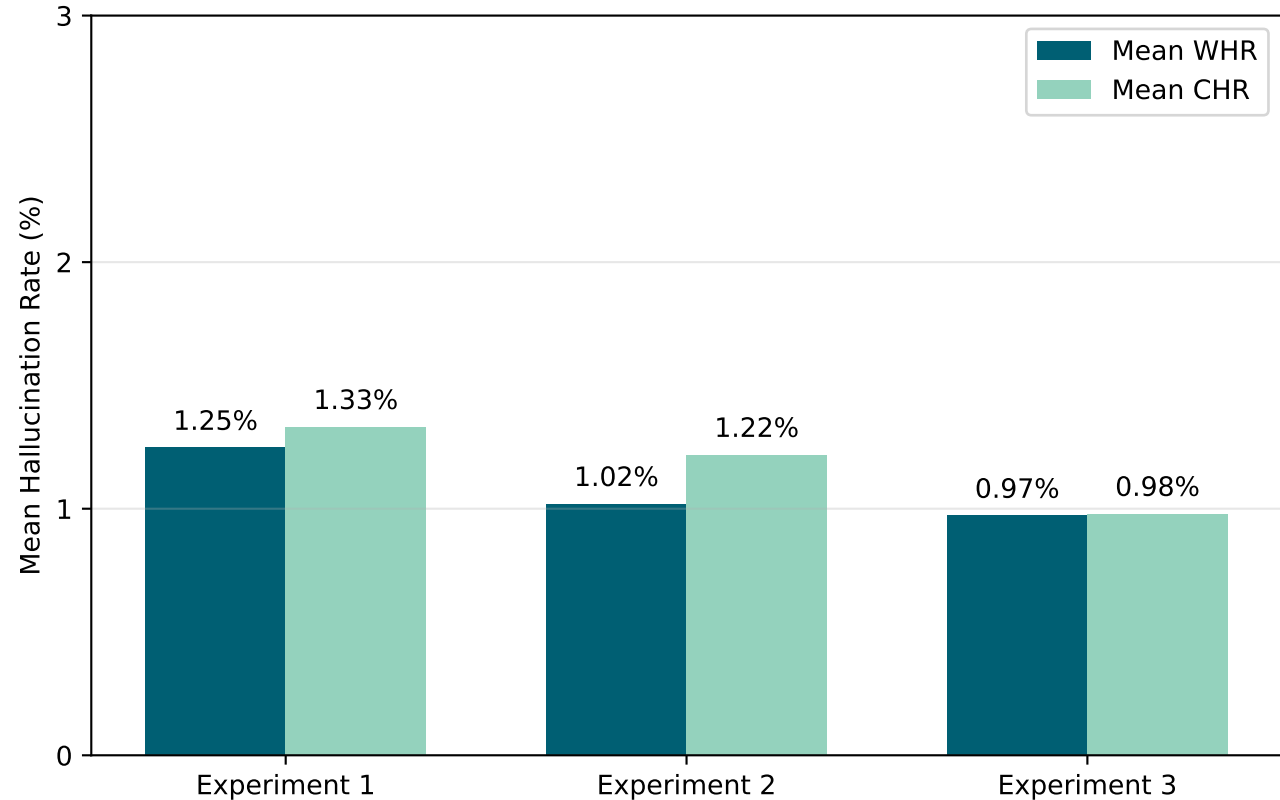
PaddleOCR-VL 1.5 Mean Hallucination Rate
