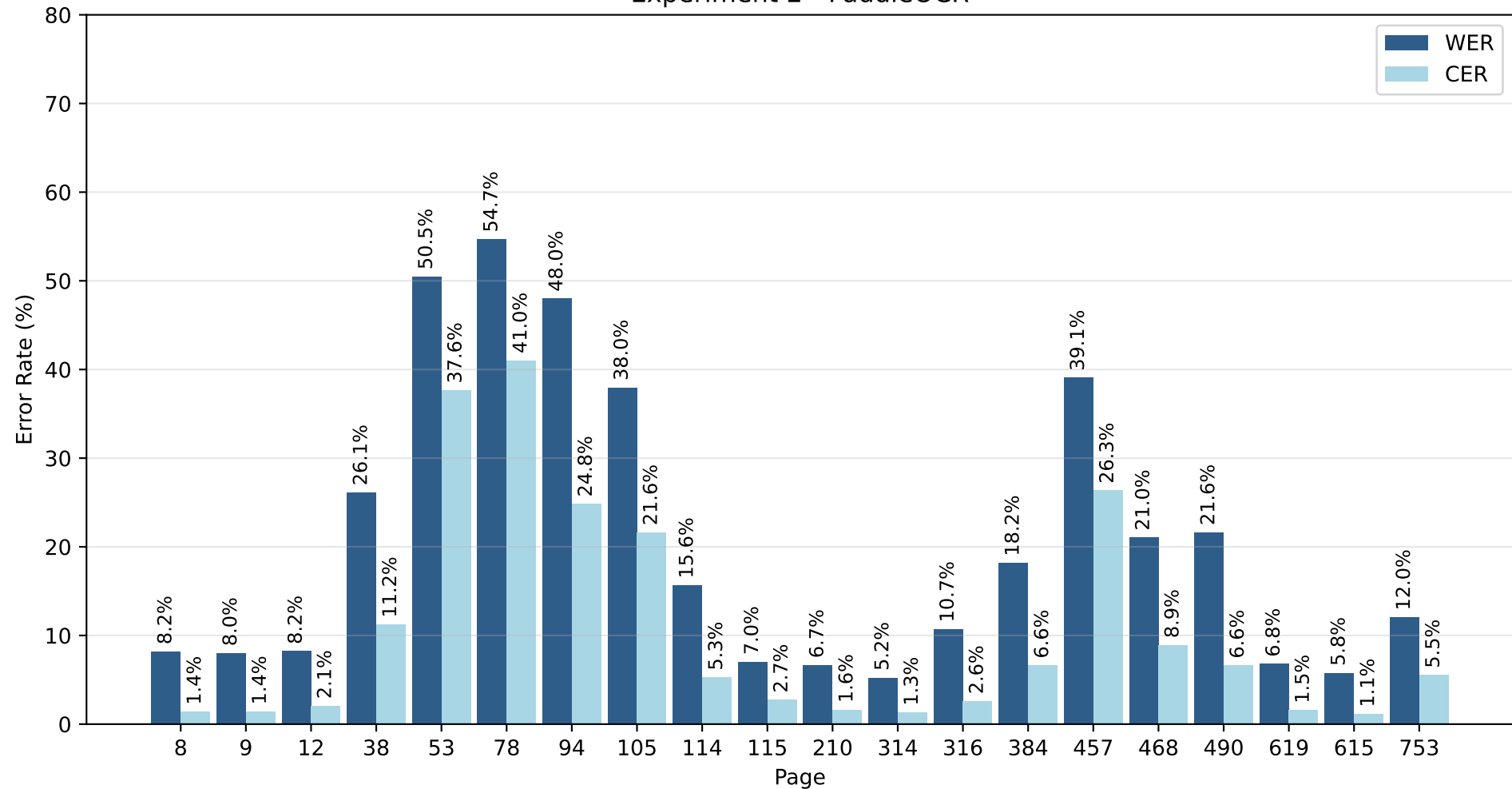
Experiment 2 - PaddleOCR
