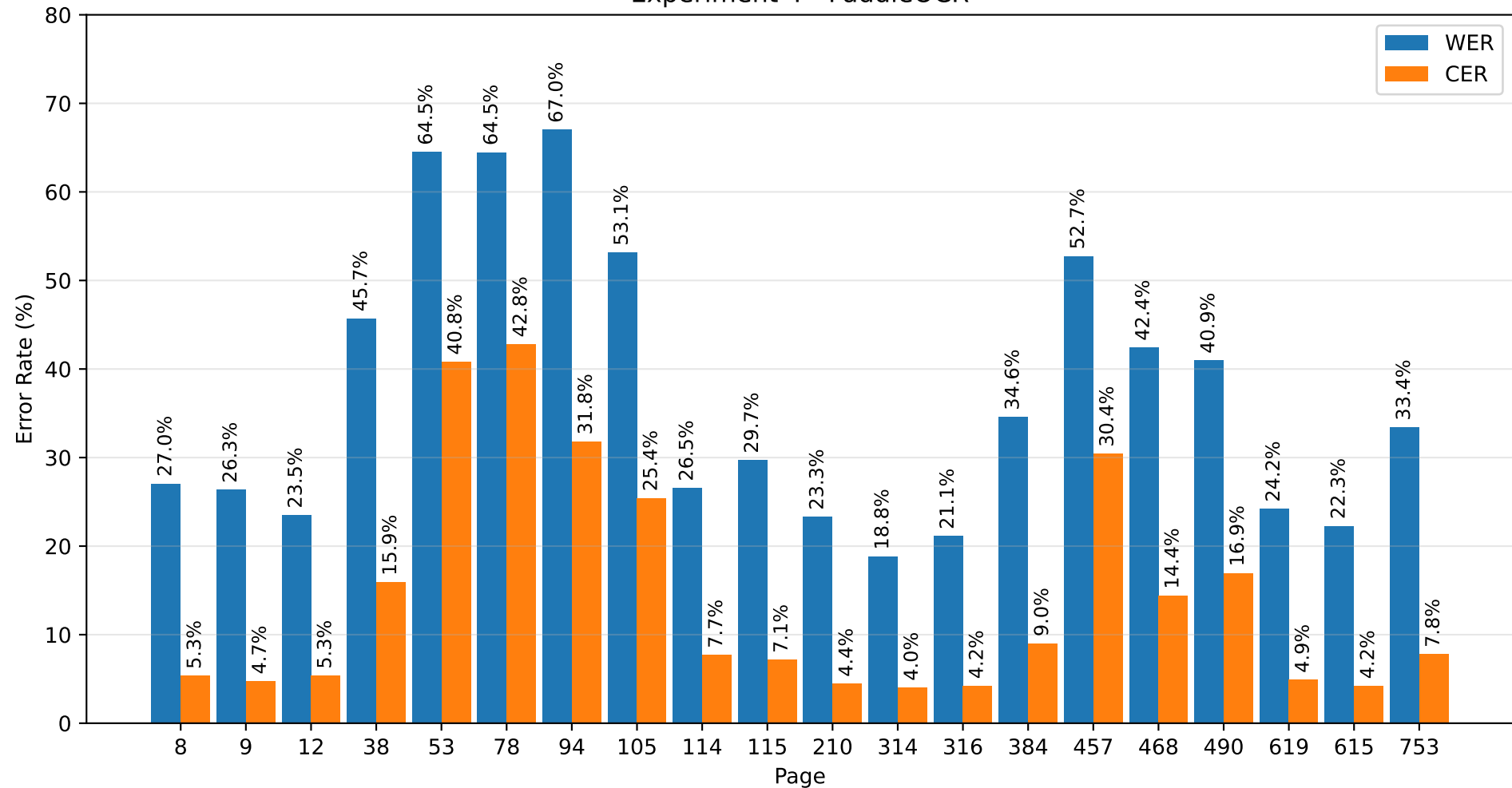
Experiment 4 - PaddleOCR
