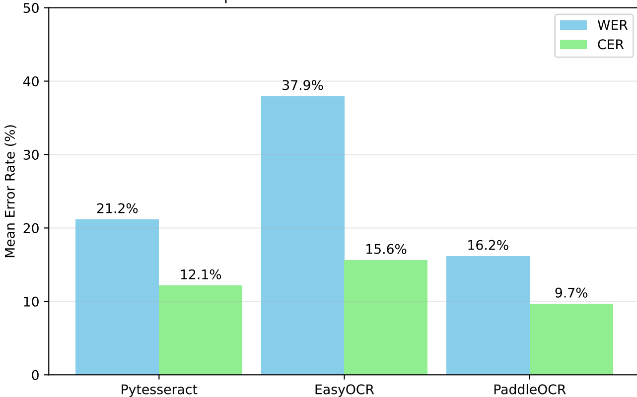
Experiment 1 - Mean WER and CER
